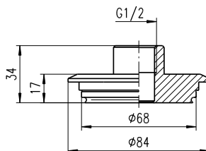
zfl / VA - TP16 VARIVENT - Flansch d=68mm
